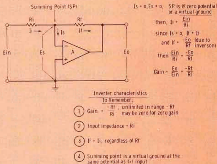
Fig. 2 The Op Amp inverting amplifier configuration
