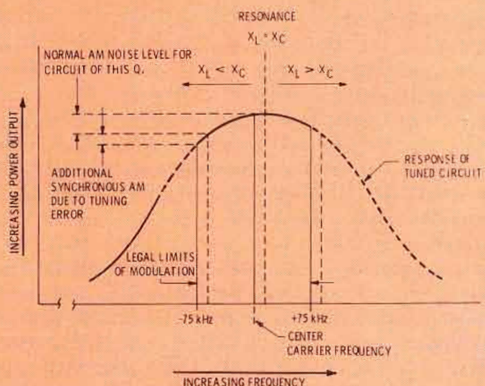
Fig. 5 A tuned circuit generating more synchronous AM than is necessary for its given bandwidth. When modulating on negative peaks, the carrier is well into the passband skirt where power falls off rapidly and additional AM noise is caused.
